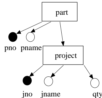
Figure 10. An invalid view schema obtained by dropping supplier.
