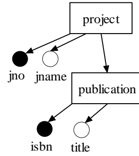
Figure 13. An ambiguous view schema.
