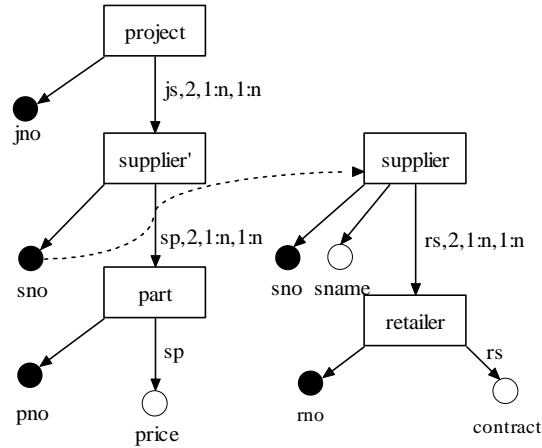
Figure 14. An ORA-SS schema diagram.
