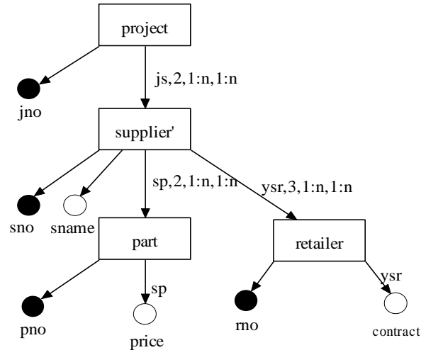
Figure 18. An invalid view schema by joining supplier' and supplier .
