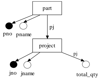
Figure 7. An ORA-SS view dropping supplier in Figure 5.
