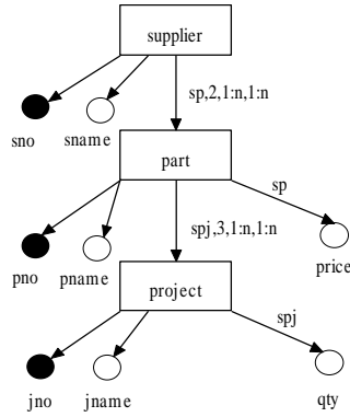
Figure 19. An ORA-SS source schema.
