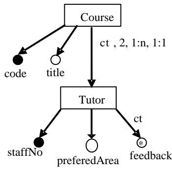
Figure 30. Changes in participation constraints due to the application of a project operator.
