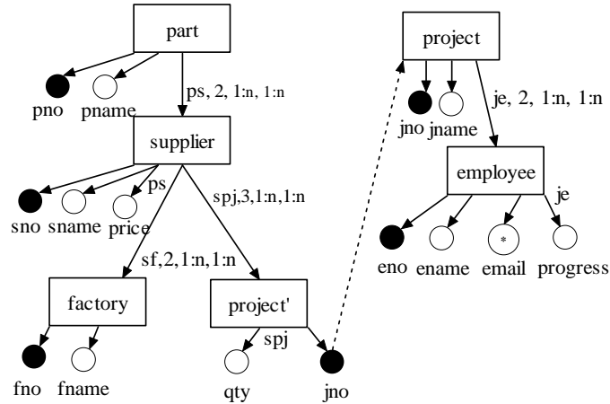
Figure 1. An ORA-SS source schema.
