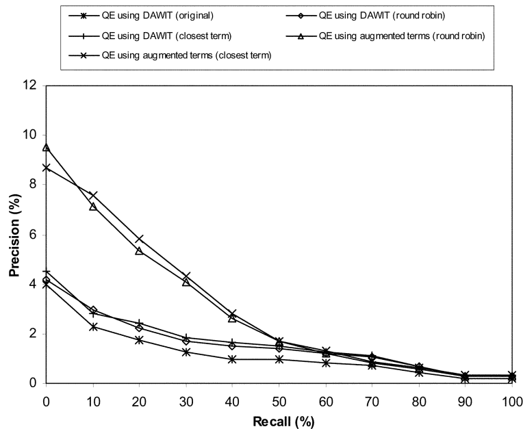
Figure 5. Precision as recall is varied (precision/recall graph).
