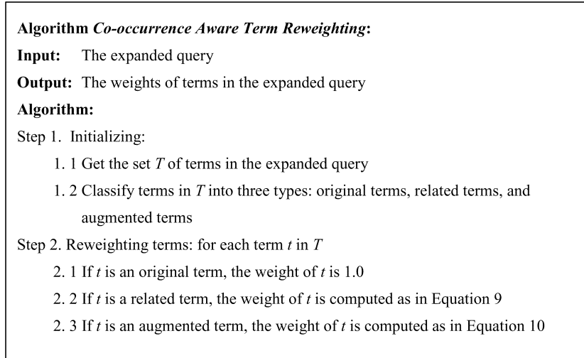
Figure 3. The algorithm for reweighting terms in the expanded query.
