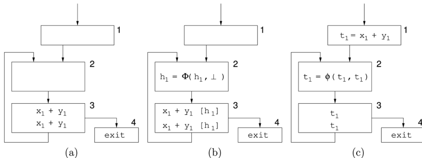
Figure 3. (a) A sample program for necessary \Phi -assignment insertion. (b) After Rename . (c) After CodeMotion .
