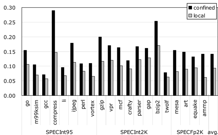
Figure 5. The number of \Phi -assignments in our locality-based SSAPRE after exploiting confined expressions and local expressions. The numbers are normalized to the original SSAPRE.
