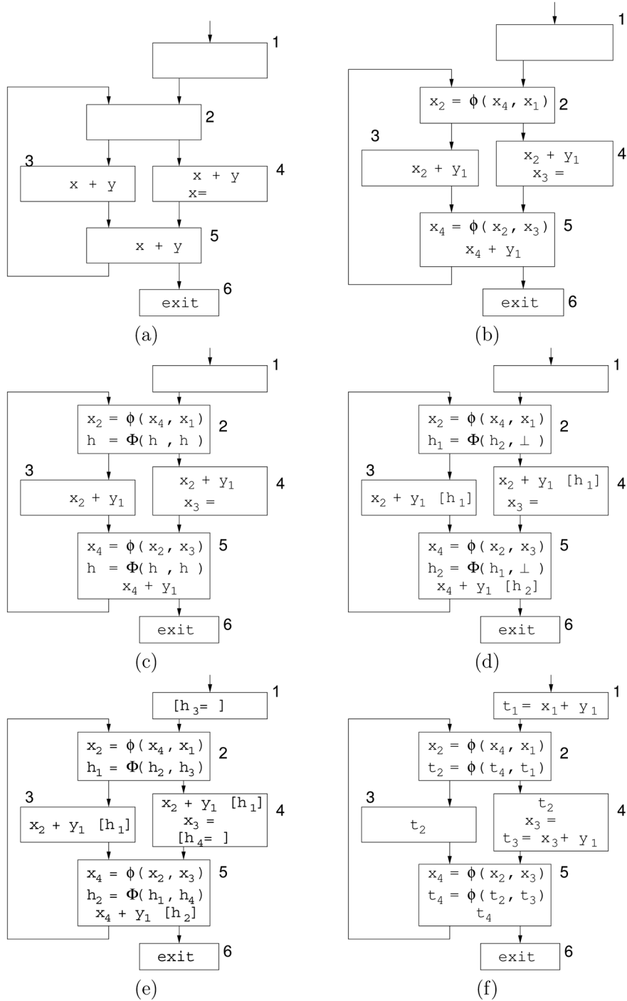
Figure 1. (a) A sample program. (b) The sample program in SSA form. (c) After \Phi -Insertion. (d) After Rename. (e) After Finalize. (f) After CodeMotion.
