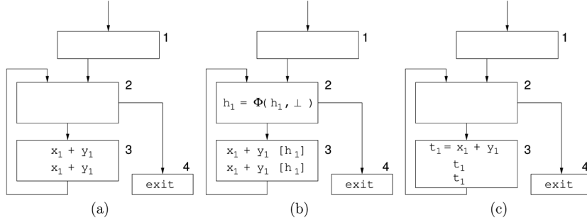
Figure 2. (a) A sample program for spurious \Phi -assignment insertion. (b) After Rename . (c) After CodeMotion .
