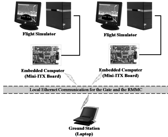
Figure 8. UAV control system architecture for multi-vehicle testing.
