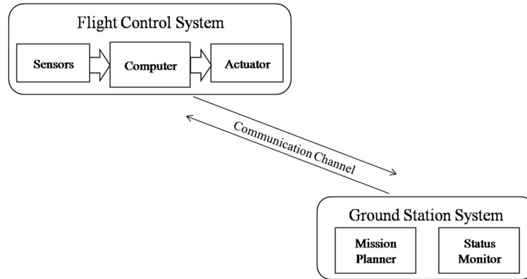
Figure 3. Constitution of the UAV control system.
