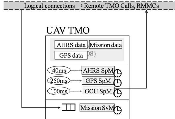
Figure 4. Design of the UAV TMO.
