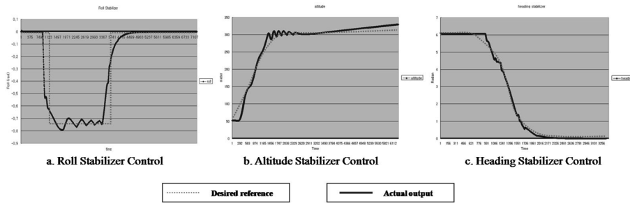
Figure 11. Stability control.
