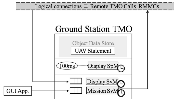
Figure 5. Design of the Ground Station TMO.
