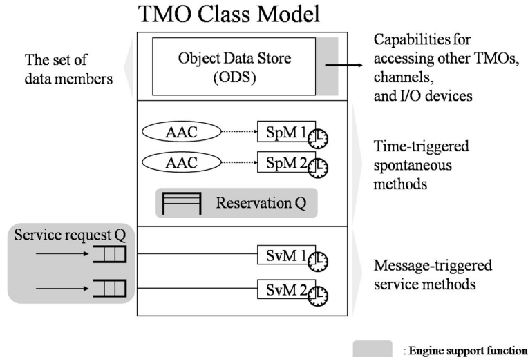
Figure 1. Structure of TMO class model.
