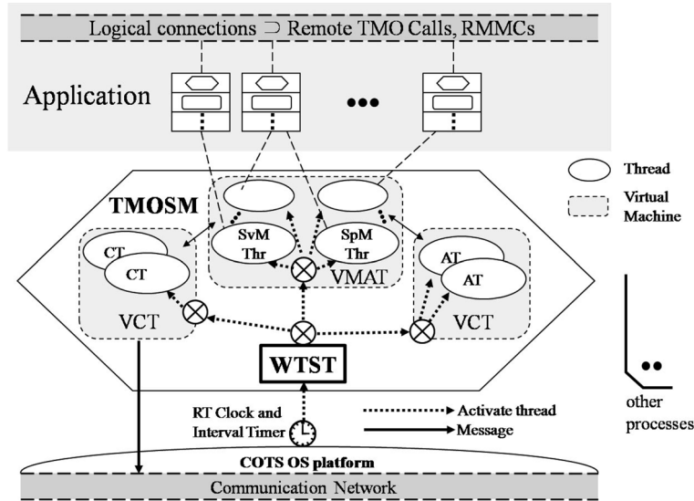
Figure 2. TMOSM architecture.
