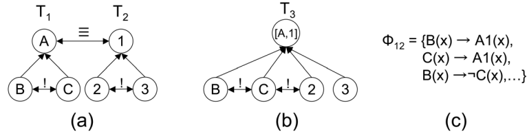
Figure 1. Given the Alignment in (a), the Merge in (b) Violates All the Described Desiderata, Except for D5 (Closure). The Merge in (c) Shows a Violation of D5.
